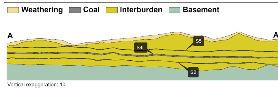
Figure 7: Matla cross-section
